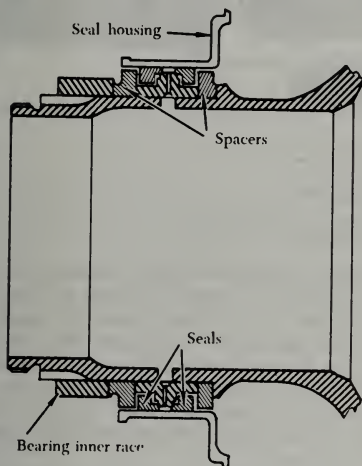
FIGURE 1-67. Carbon oil seal.
